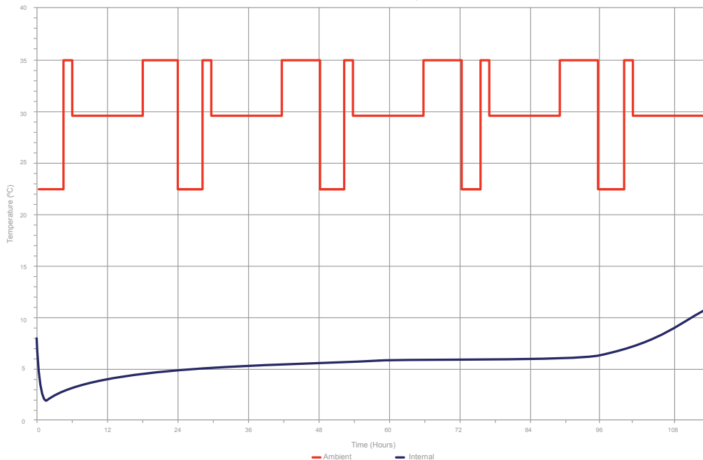
Series 4 - 2896, with Pelican Case, ISTA Summer Thermal Performance (Control Set: ISTA 7D Summer Profile, No Payload, -18°C TIC Conditioning, 23 Minute TIC Staging) Source: MTS Lab 22 February 12
